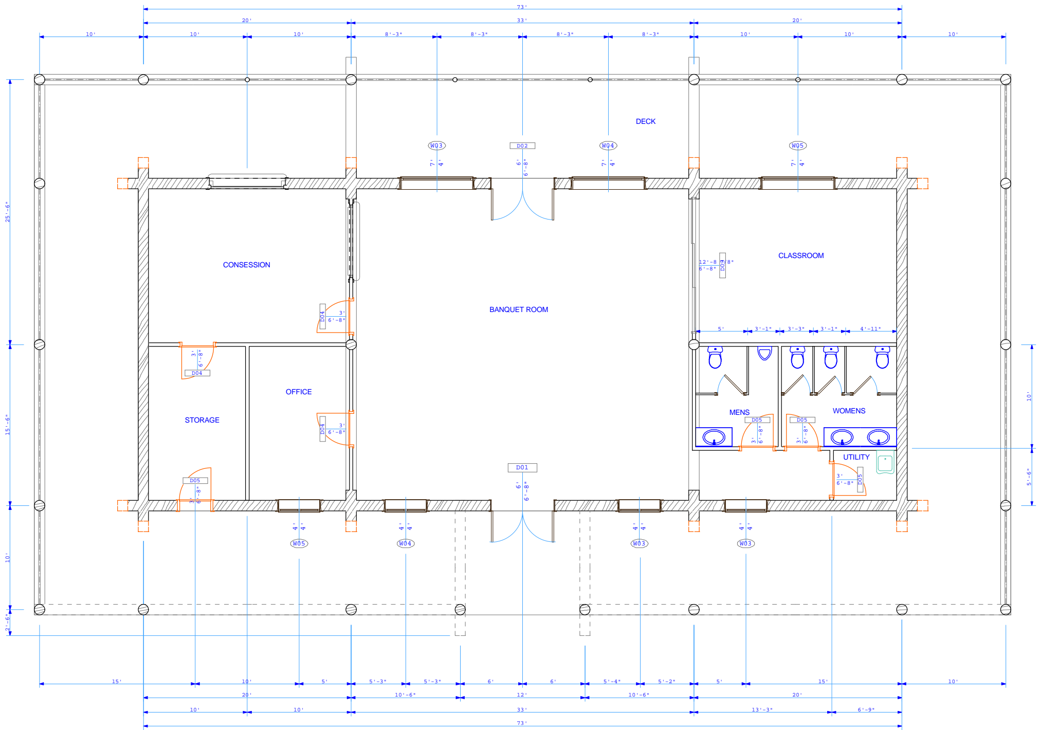
PROPOSED SOCCER CLUBHOUSE PRELIMINARY MAIN FLOOR
